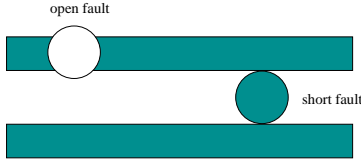
Figure 1: An open fault is formed due to loss of mass; a short fault is formed due to augmentation of mass.
