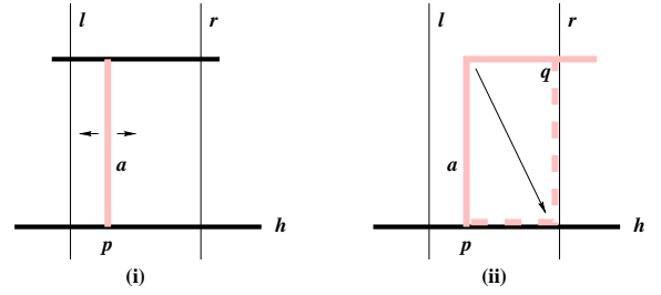
Figure 3: (i) If augmenting path a connects two parallel edges, then l(G) remains constant when a slides horizontally, and for at least one direction lbridges(G) does not increase. (ii) Otherwise, a can be re-embedded along the Hanan grid lines.
